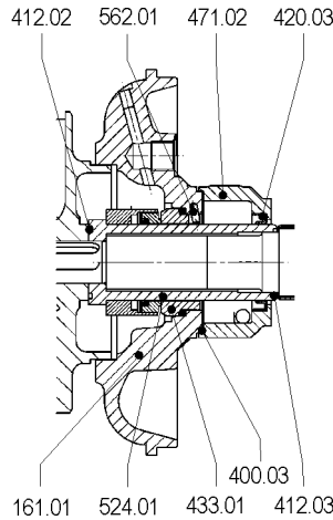
Unbalanced mechanical seal with quench and shaft seal ring
