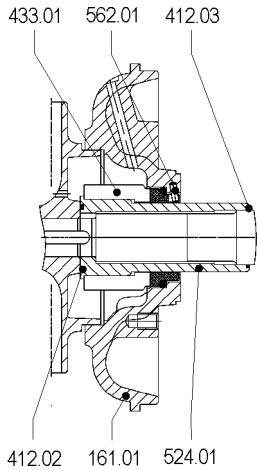
Balanced single mechanical seal
