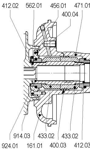
Balanced multiple mechanical seal in back-to-back arrangement
