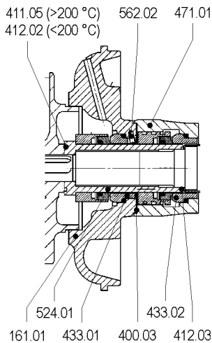
Unbalanced multiple mechanical seal in tandem arrangement
