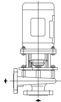
Vertical installation
